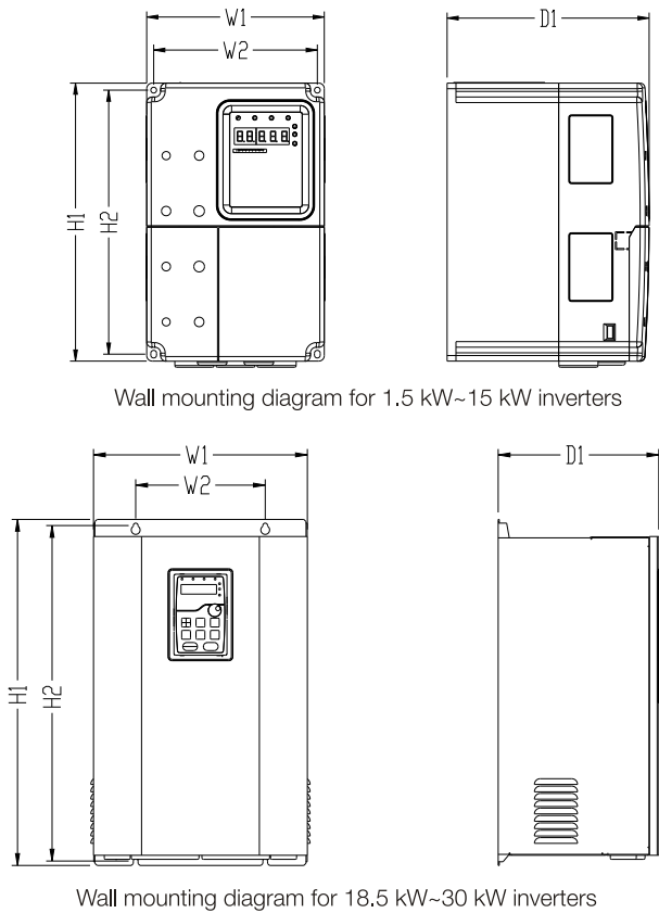
Wall-mounting dimensions for 380V inverters (unit: mm)
